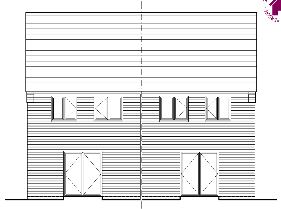
Rear Elevation
